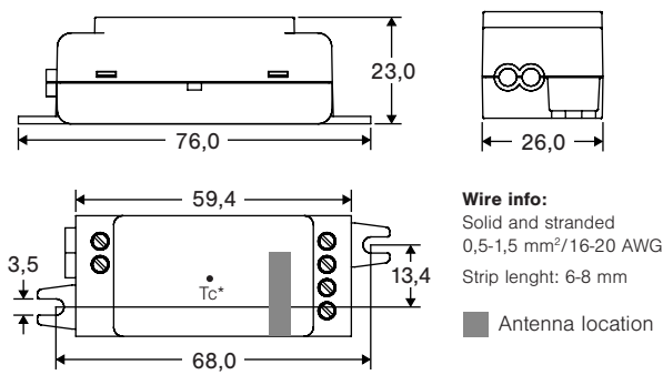
Dimensions are in mm. * Tc point is on bottom side
